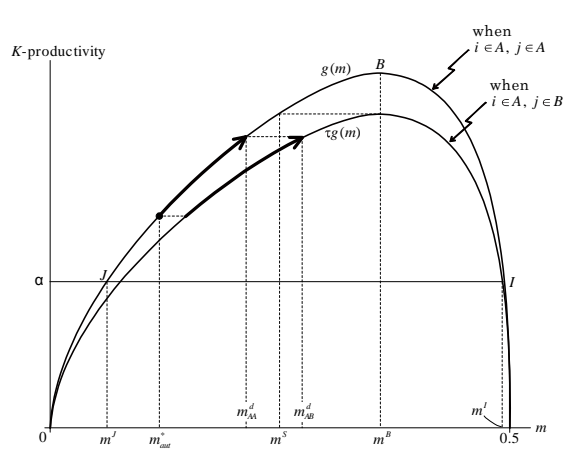
Figure 10: Transition process, Phase 2 (with inter-regional interactions): g(m^d_{AA}) = g(m^d_{AB}) > g(m^*_{aut})
